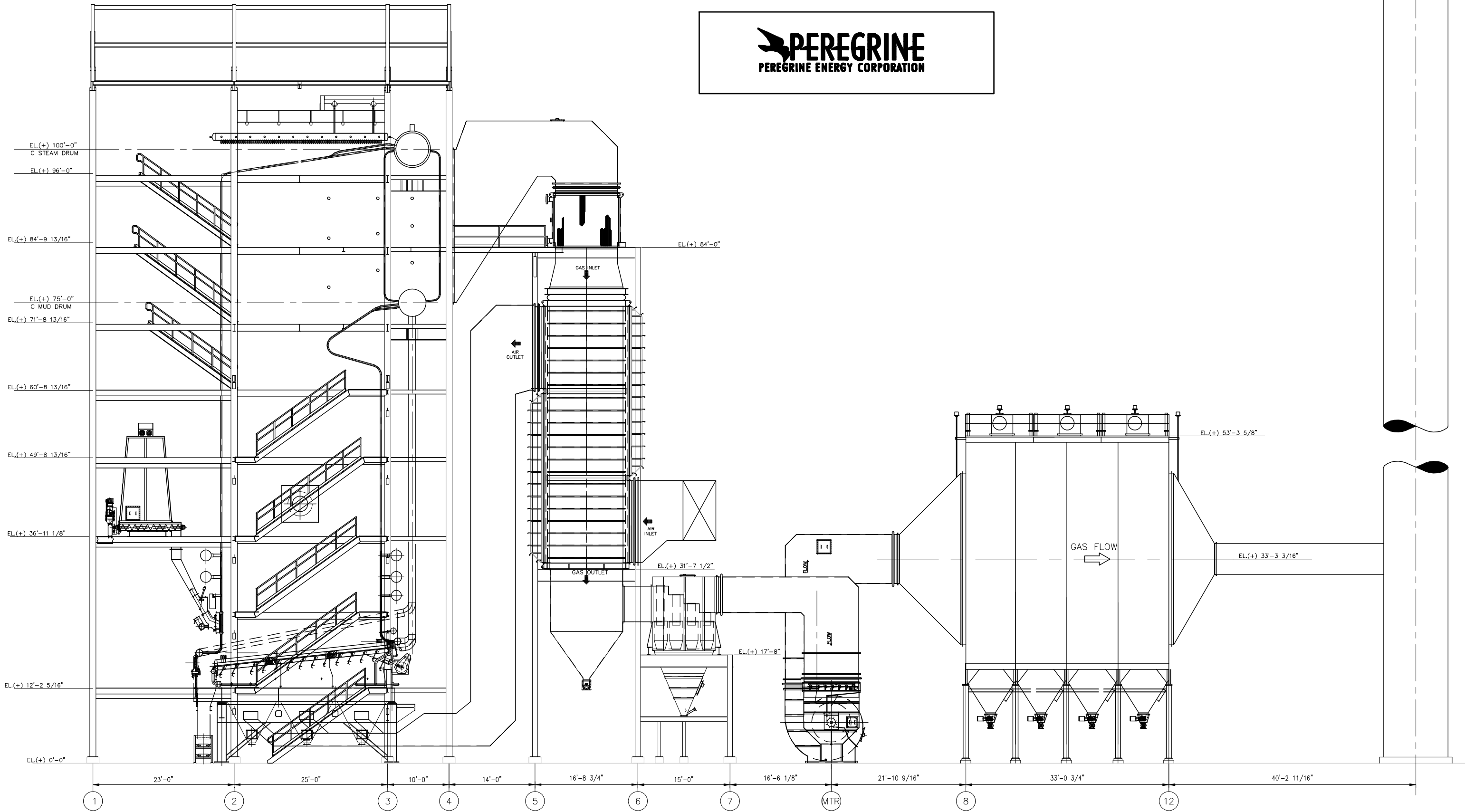
BOILER SYSTEM ELEVATION SCALE: 1/8" = 1'-0"
